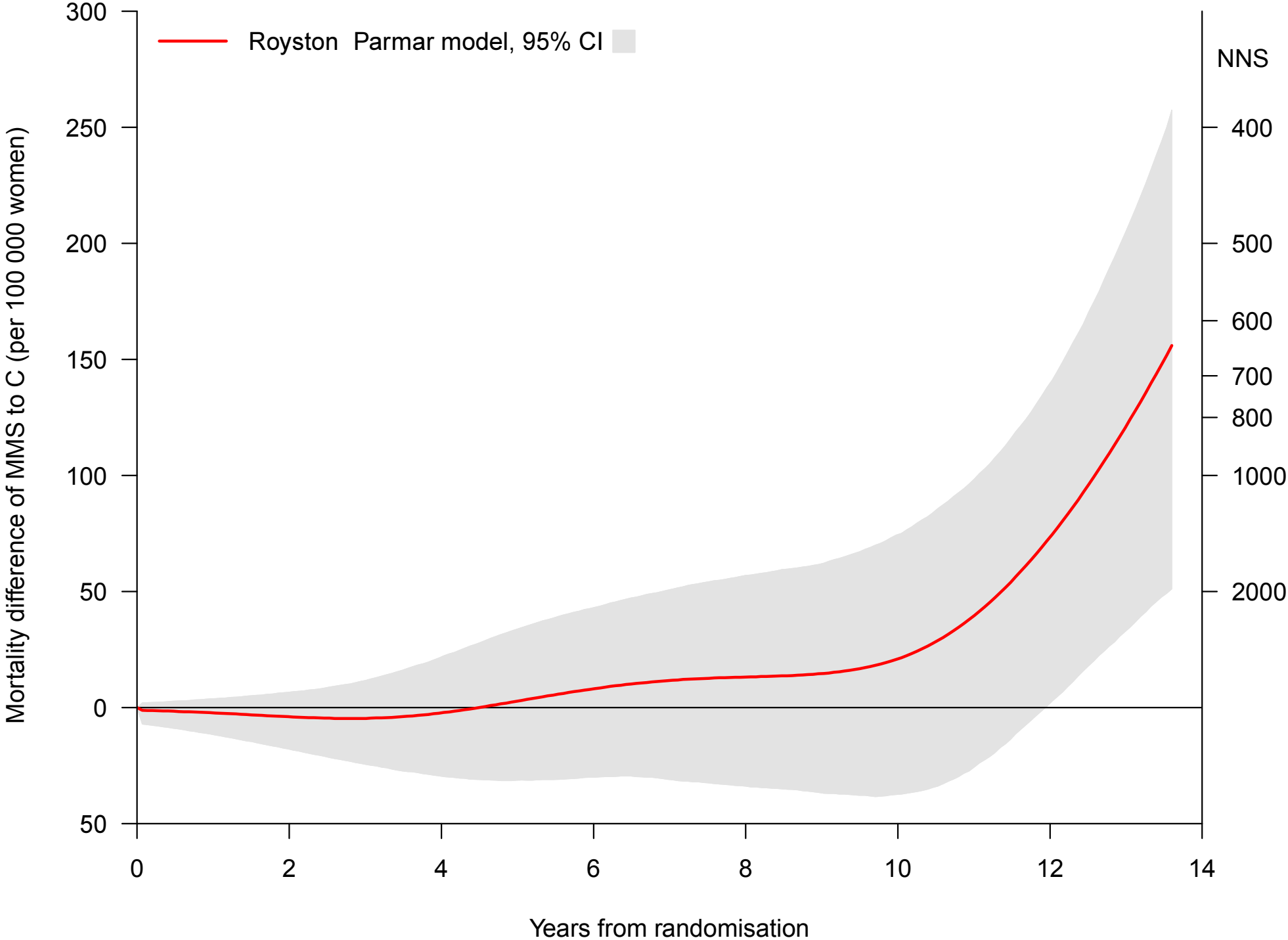
Figure 5: Mortality difference and numbers needed to screen (NNS) to prevent one death from ovarian cancer.
