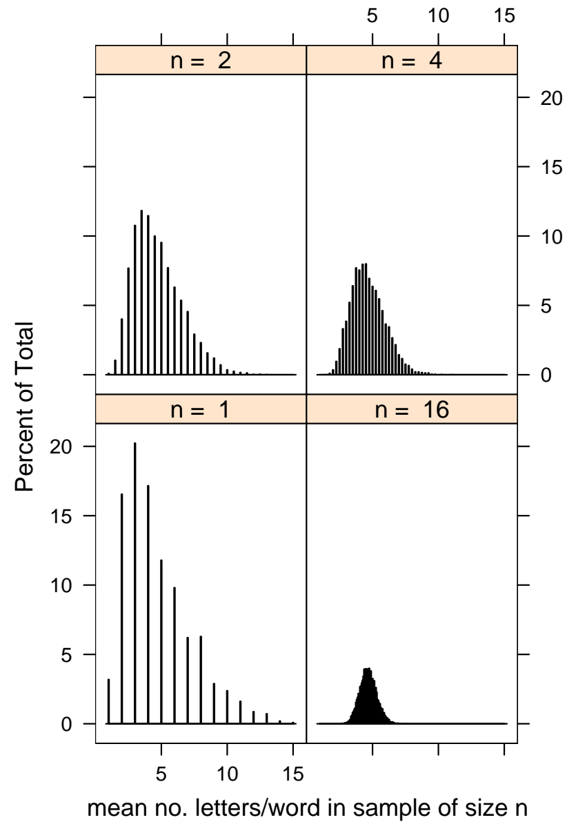
Figure 2: Another illustration of Central Limit Theorem (harder?) at work
