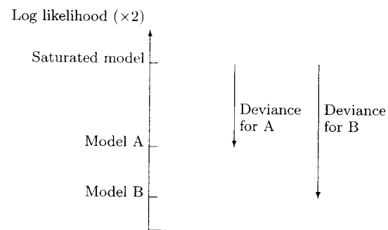
Fig. 24.1. Relationship between deviance and log likelihood
