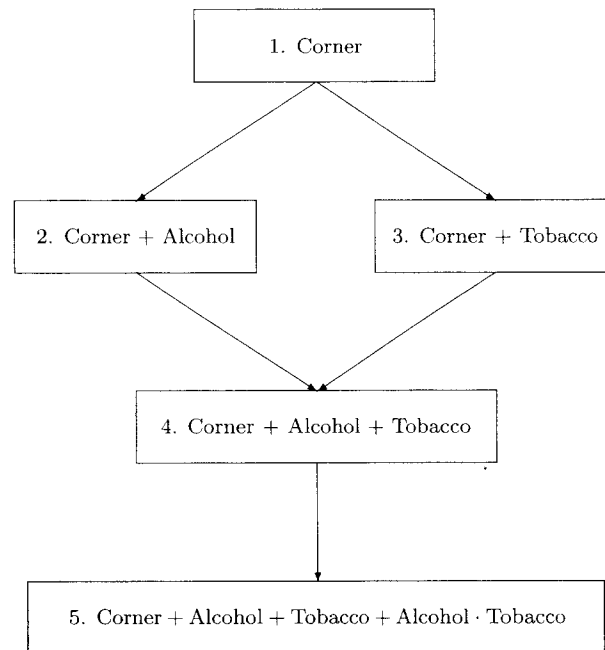
Fig. 24.2. Nesting of models.
